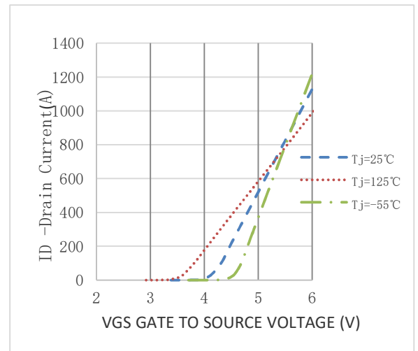
Figure 10. Transfer Characteristics
