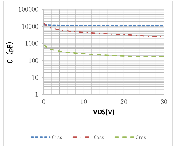
Fig.2 Capacitance Characteristics
