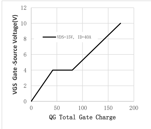
Fig.1 Gate-Charge Characteristics
